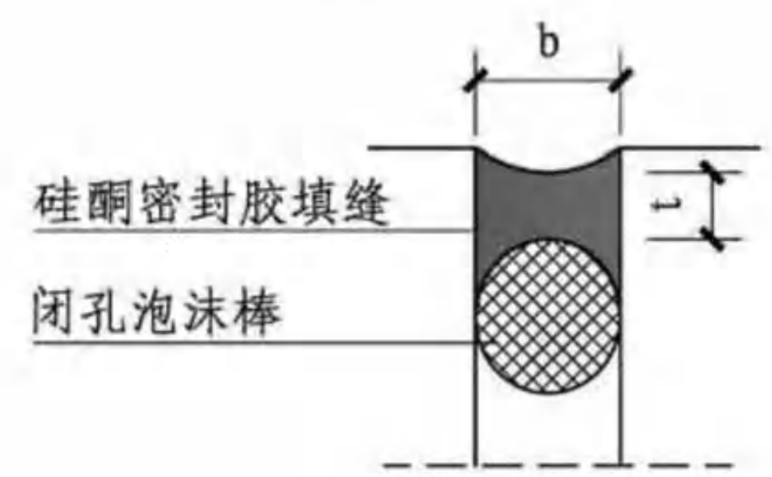
A 硅酮密封胶填缝
