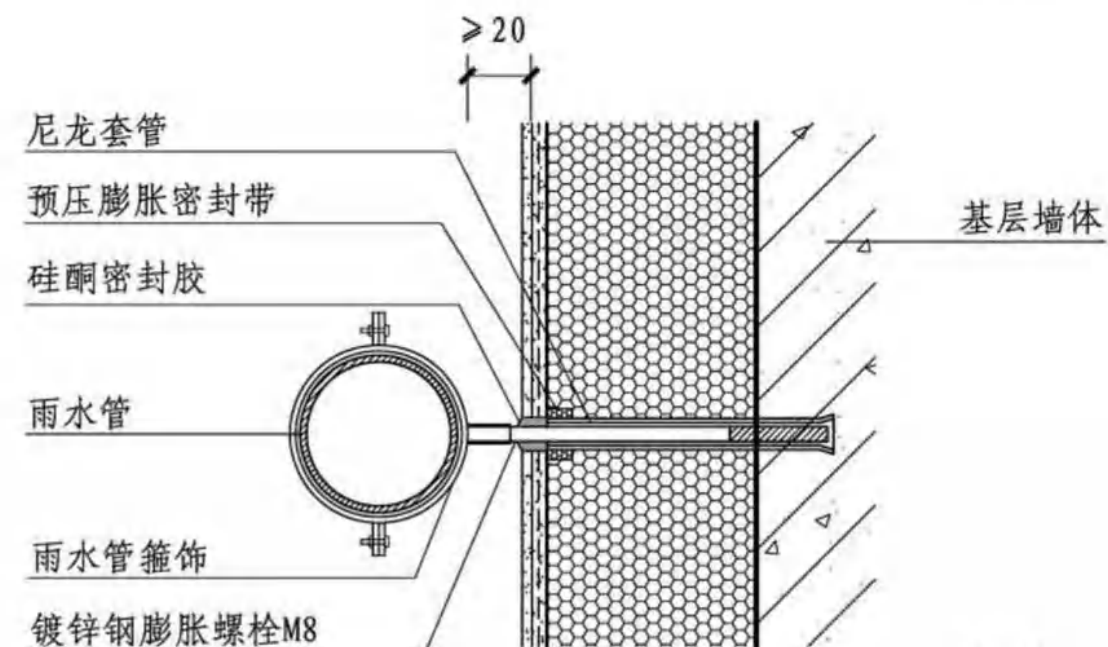
2-2
